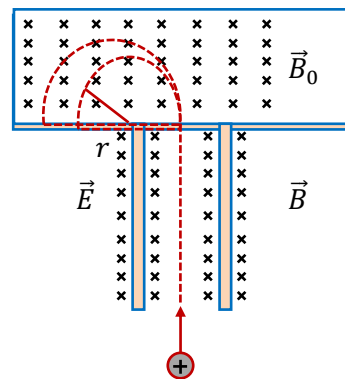
Figure: A Bainbridge mass spectrometer
